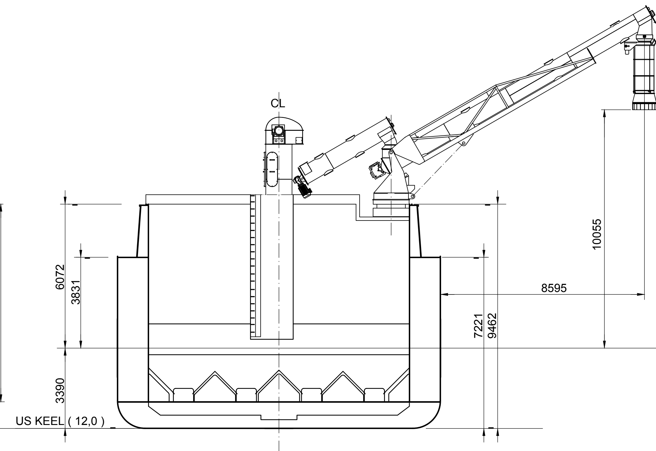
BALLAST AT PLIMSOLL MARK
